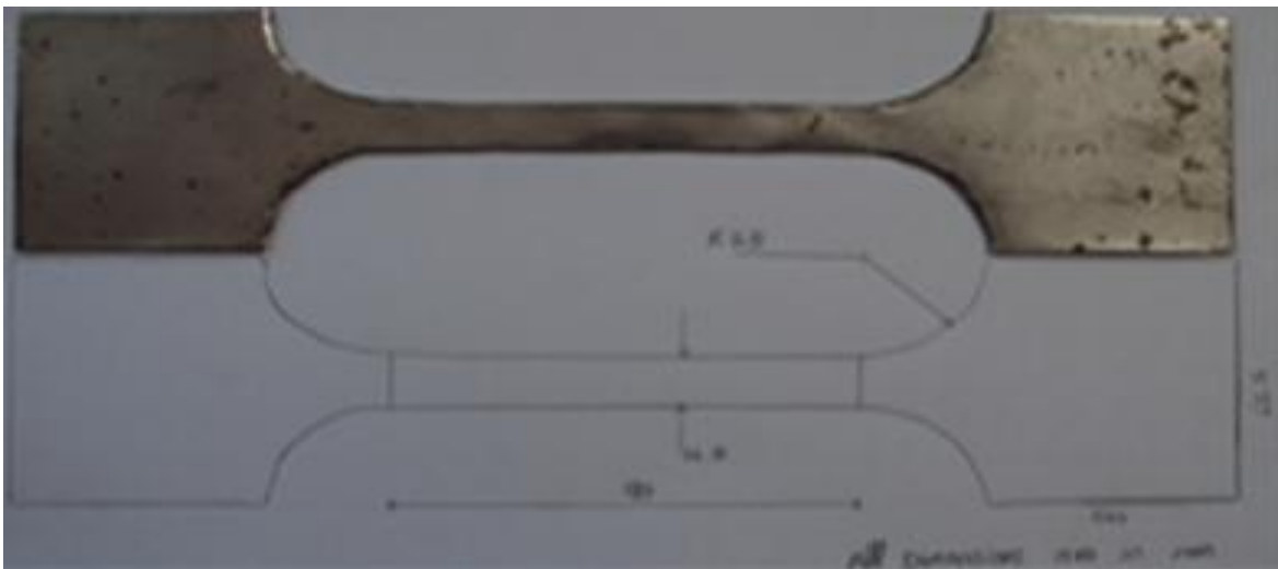
Fig. 1 Coupon test Specimen based on IS Code
