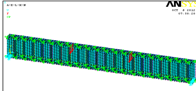
Fig. 6 Meshed test Specimen with boundary condition and loading.
