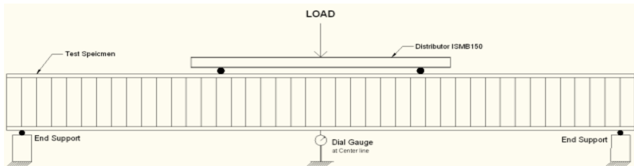
Fig. 3 Diagrammatic representation of test setup
