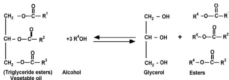
Fig.1. Transesterification of vegetable oil into mono- alkyl esters (biodiesel)
