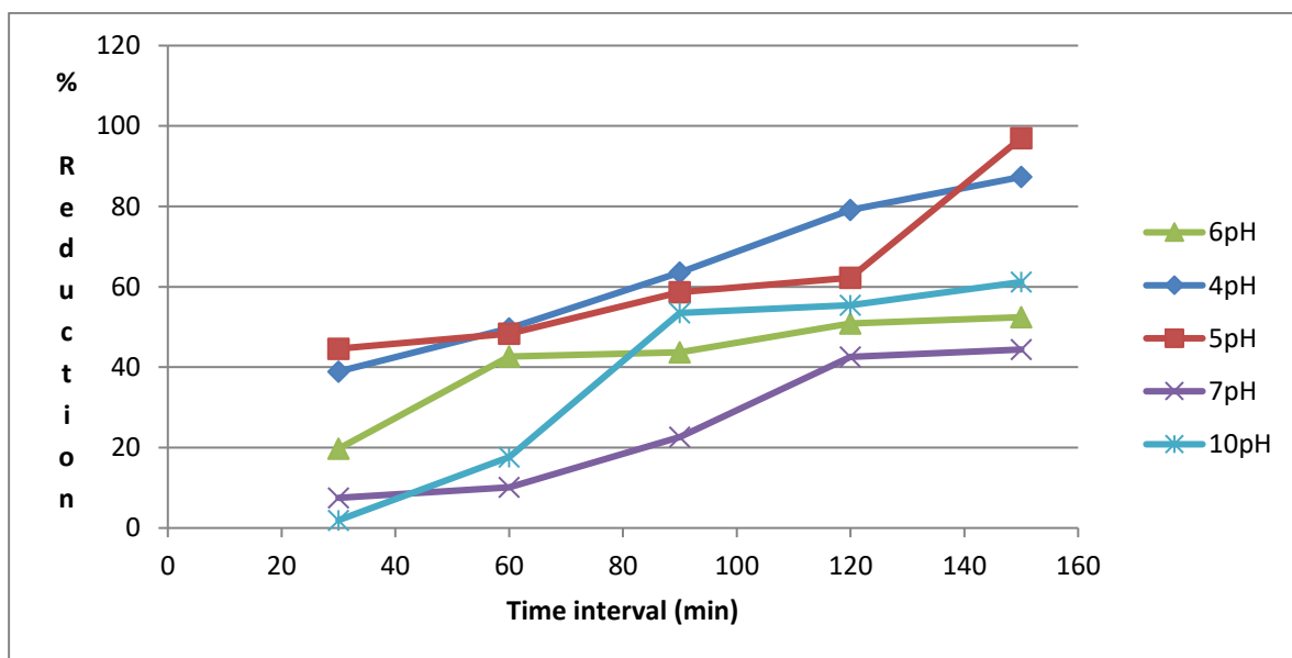
Graph.2: % Reduction vs time interval at dosage 100mg and 4ppm constant at different pH
