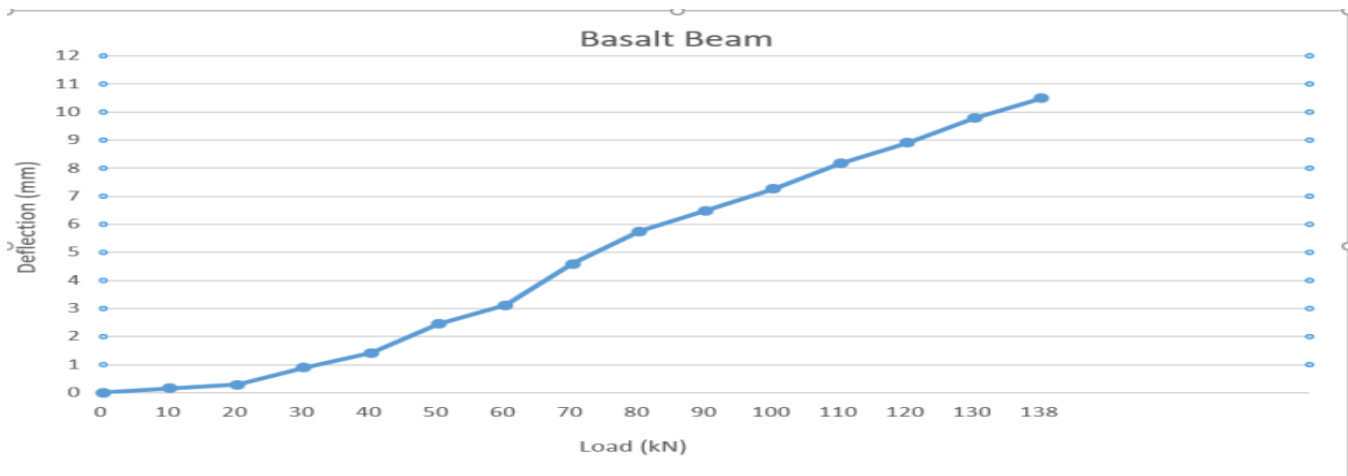
Charts 1 : Deflection vs load graph
