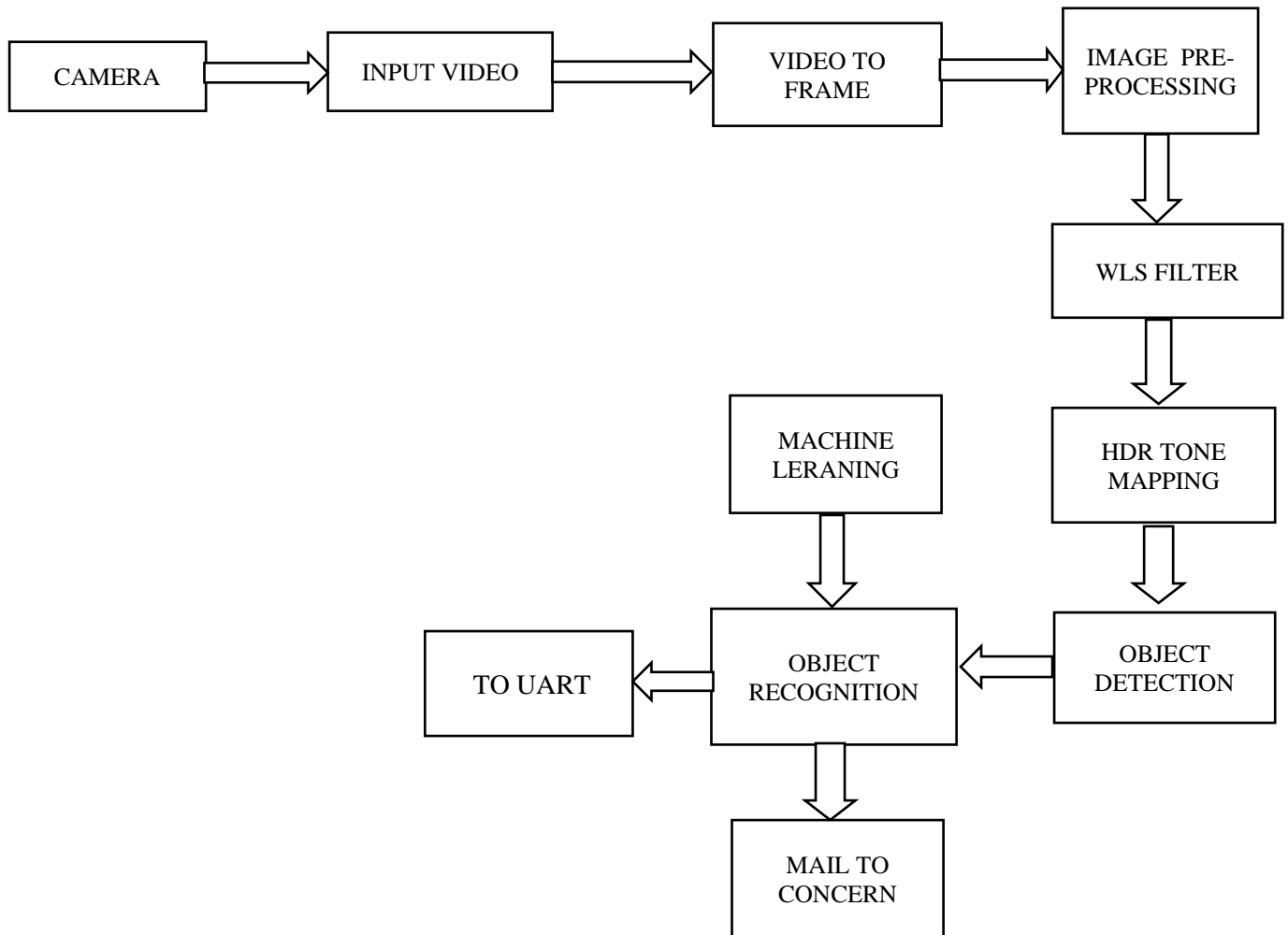
4.1 Block diagram of detection and recognition of object
